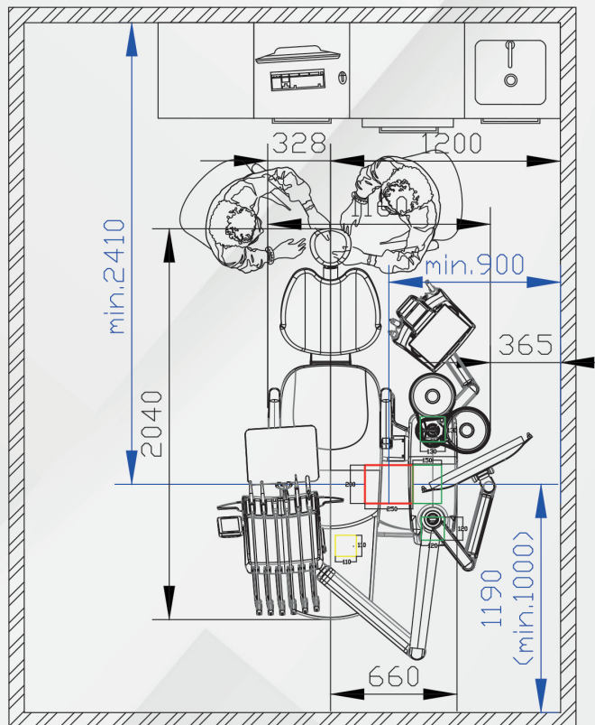
OVERALL DIMENSIONS (Measurements in millimeters)
